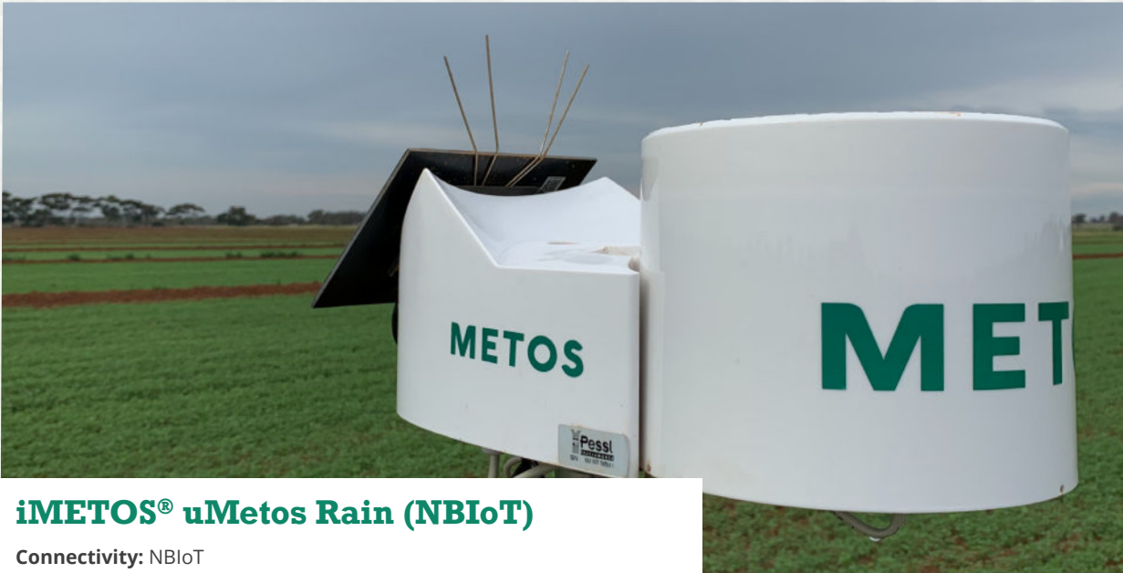
uMETOS Soil Connectivity: NBIoT
